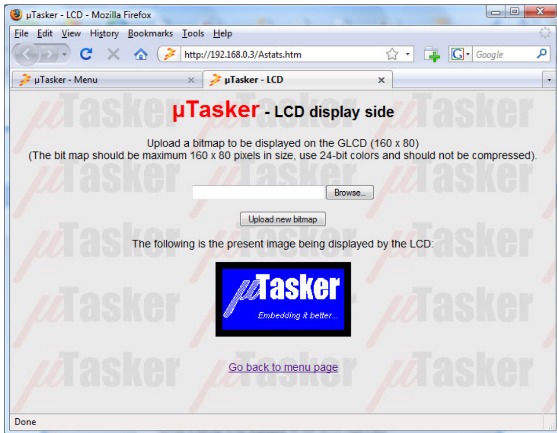
Figure 10. Temporary LCD page showing the present LCD image
