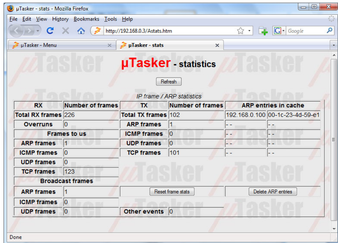
Figure 8. µTasker web server showing the statistics page
