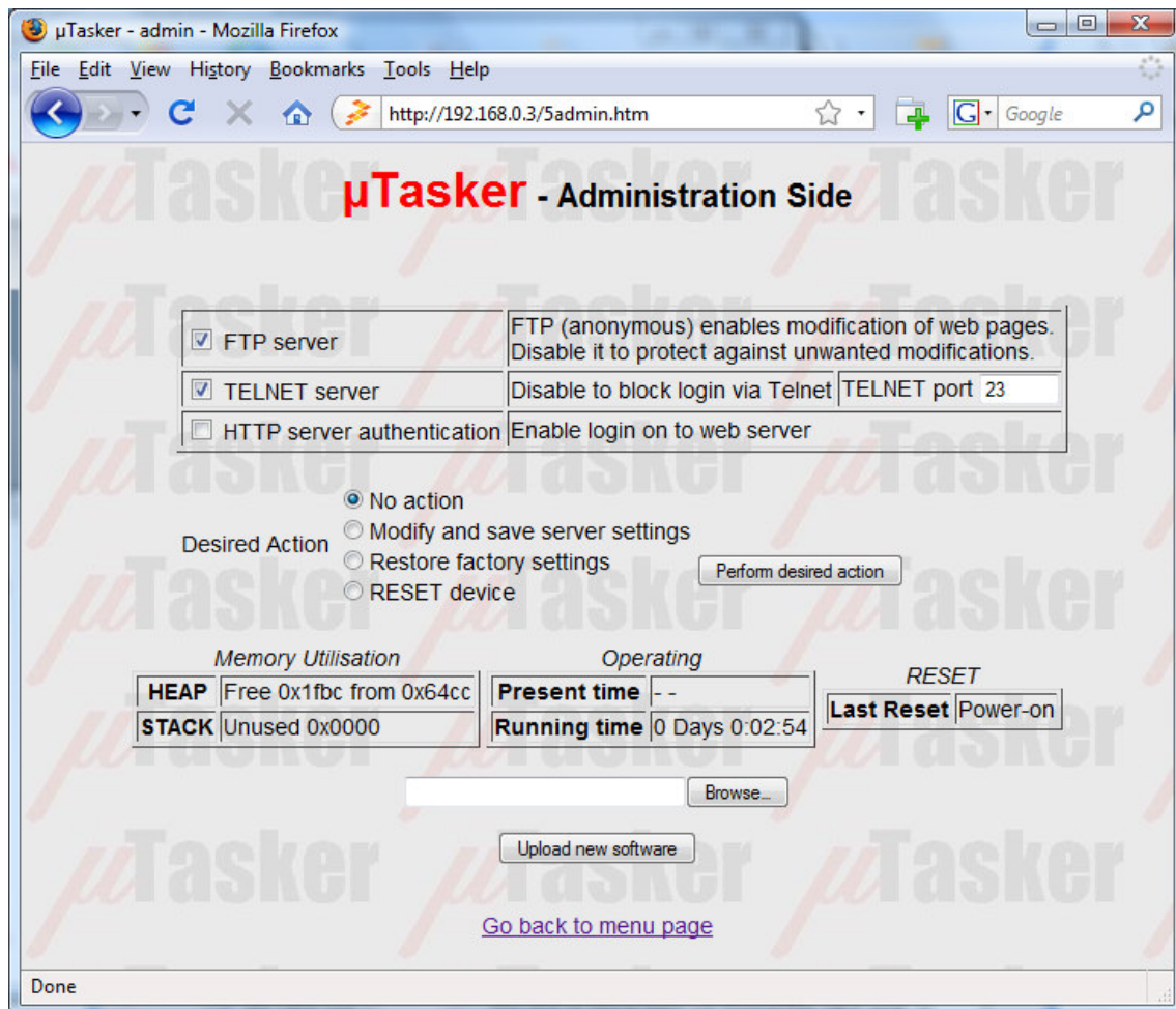
Figure 9. µTasker web server showing the administration page
