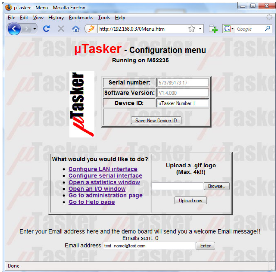
Figure 5. µTasker web server showing the menu page
