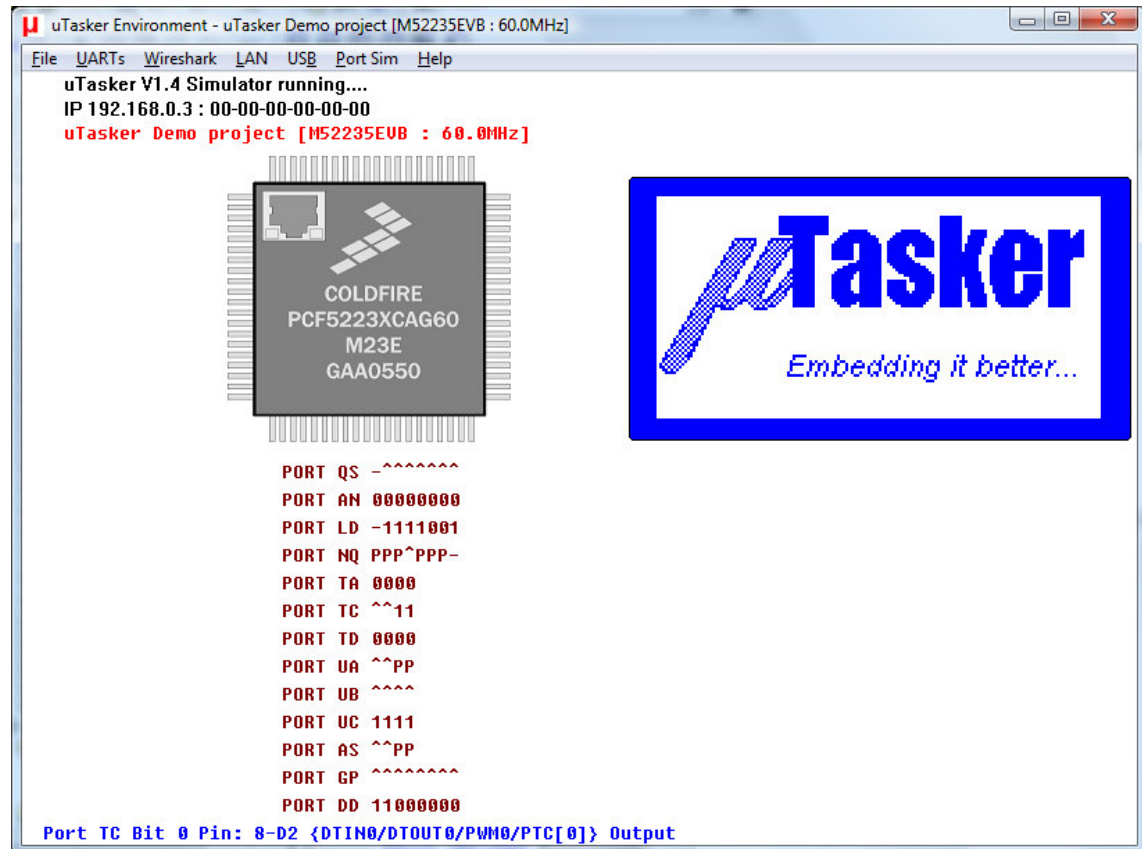
Figure 1. µTasker simulator running a M52235EVB board
