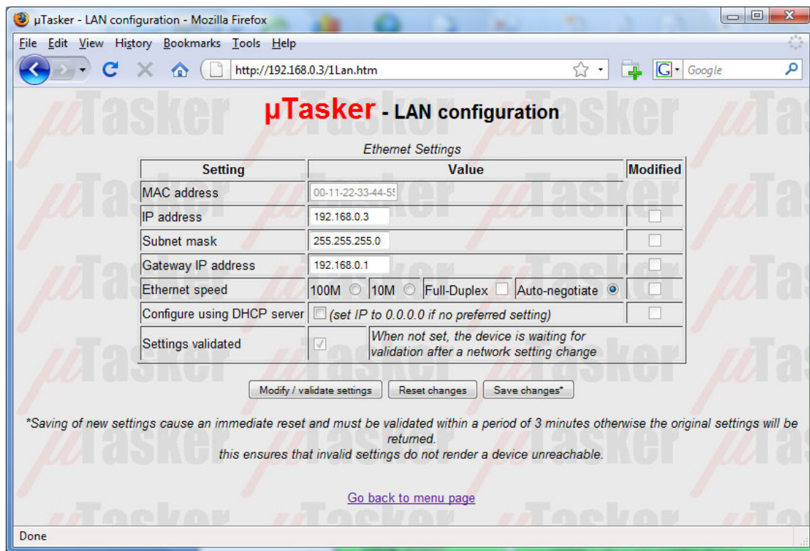
Figure 6. µTasker web server showing the LAN configuration page
