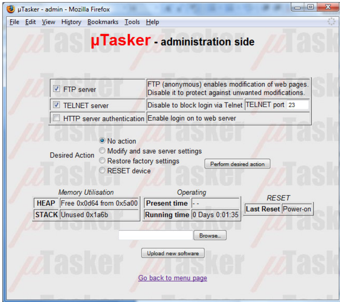
Figure 9. µTasker web server showing the administration page
