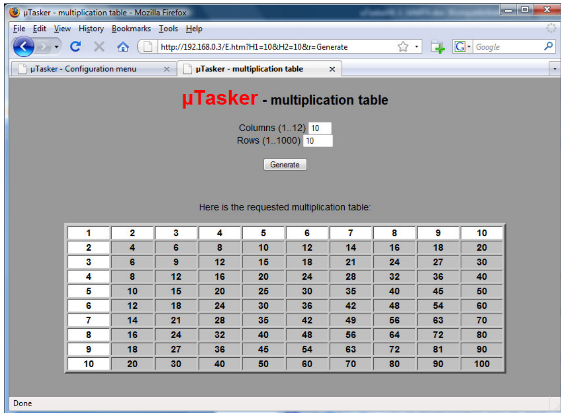
Figure 11. Dynamically generated multiplication table
